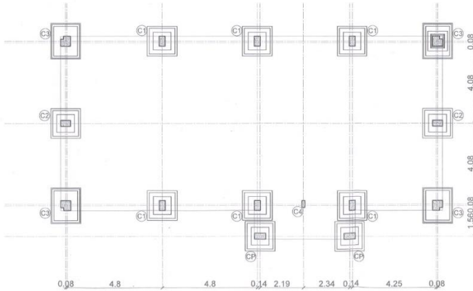
FOOTING PLAN SCALE 1:100
