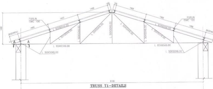
TRUSS T1-DETAILS
