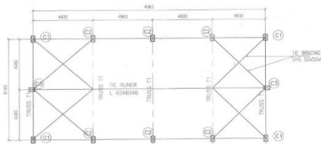
KEY PLAN FOR TRUSS
